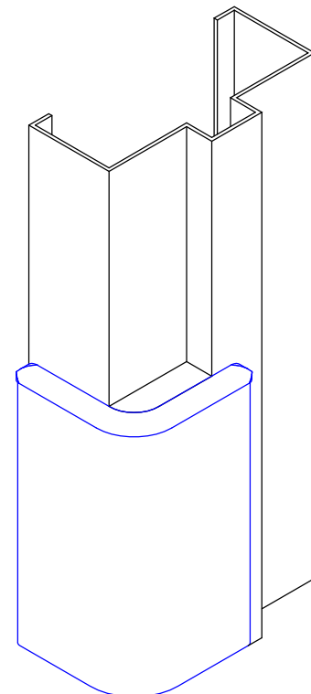
Installed View
