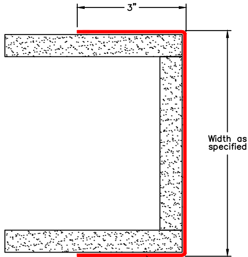
Super Duty End Wall • .050" formed aluminum • .030" polyurea coating
